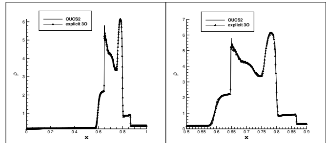
Fig. 4. Interaction of blast waves in one dimension: result at t = 0.038 . Left frame: full domain, right frame: zoomed view. Grid size: 800 cells, CFL = 0.1.
