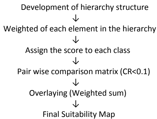
Fig. 3. Methodology of Analytical Hierarchical Process and integration of map layers.
