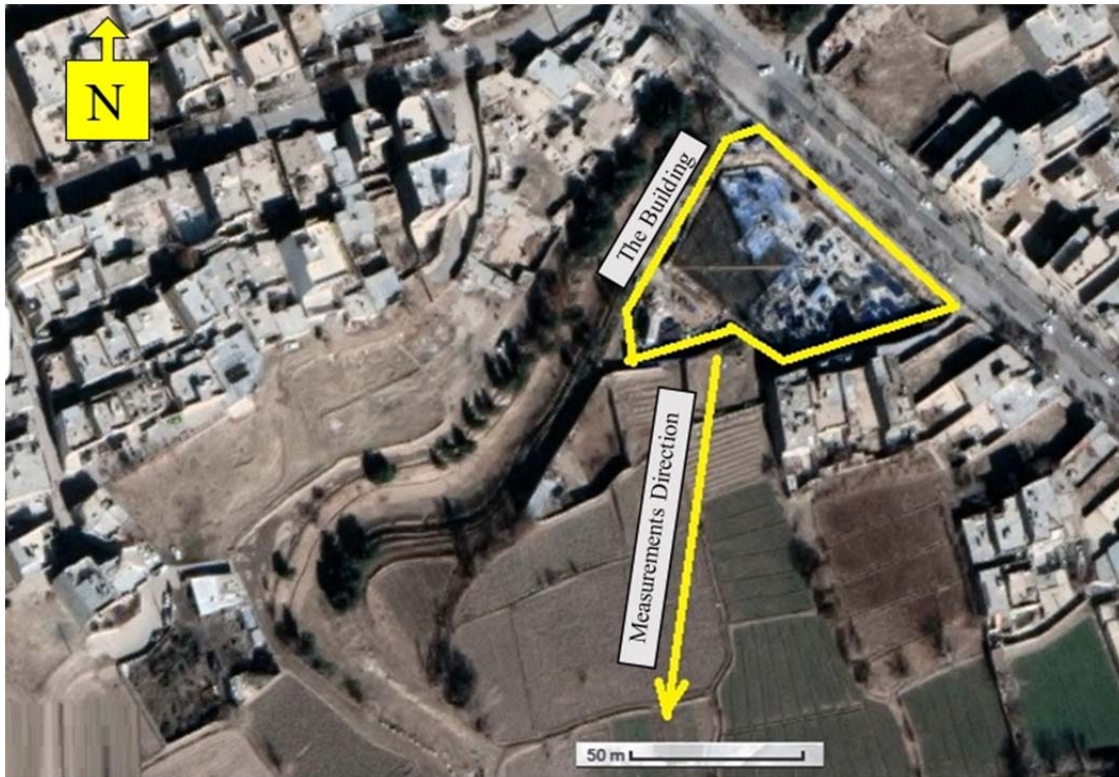
Fig. 1 The building location and Measurements Direction (Courtesy of Google MAP)
