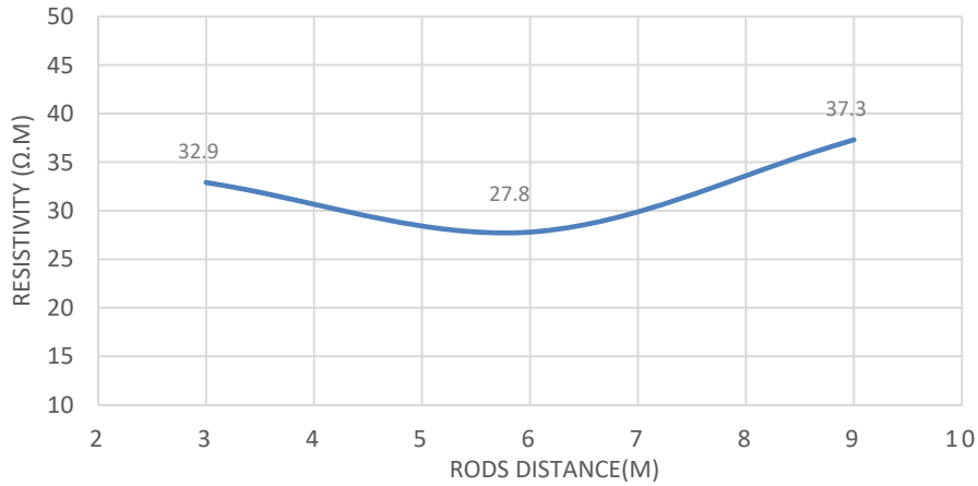
Fig. 8. Soil resistivity profile
